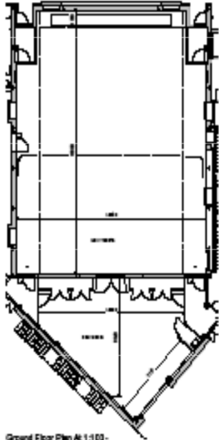
Ground Floor Plan At 1:100 - Seating Retracted
